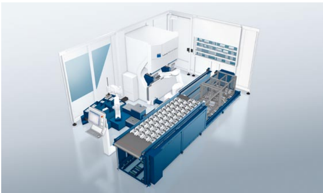
TruBend 7036 Cell Edition, BendMaster (15), LoadMaster Bend, ToolMaster Bend, and conveyor system.
